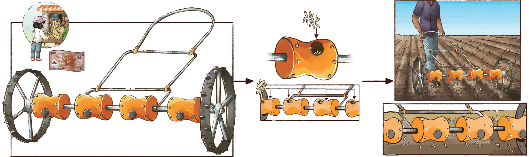
1. Four-row wheel seeder for rice
